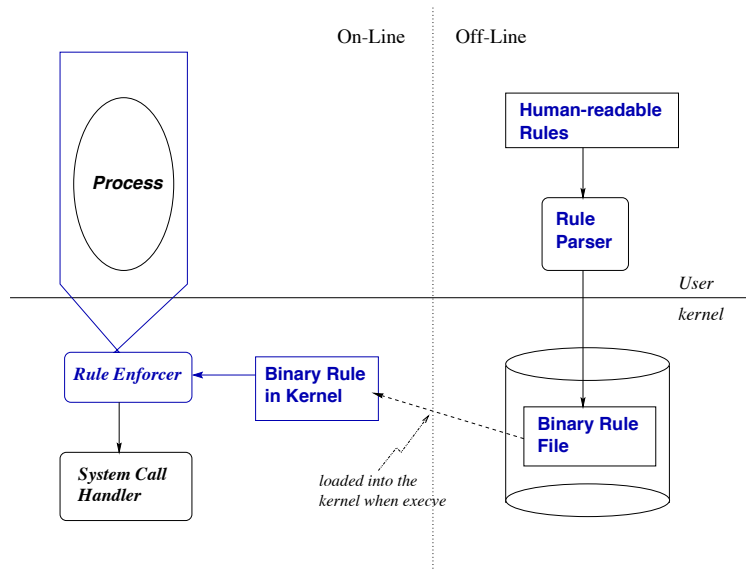
Figure 1. BlueBox Architecture
