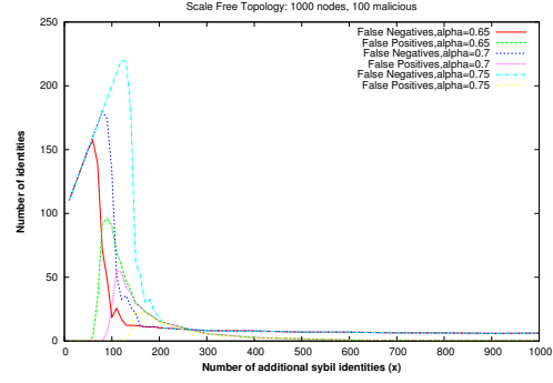
(b) Low degree compromised nodes
