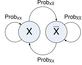
(a) A schematic representation of transition probabilities between honest X and dishonest \bar{X} regions of the social network.
