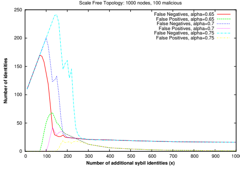
(a) Average degree compromised nodes
