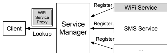
Fig. 2. System services register themselves to Service Manager and clients call their remote interfaces with proxies.
