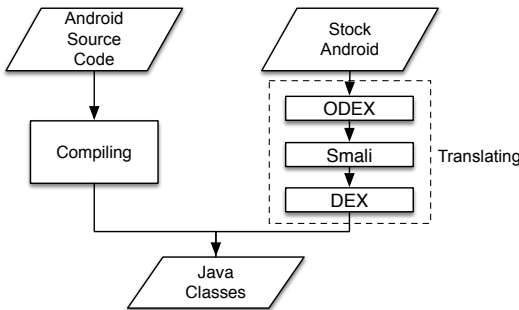
Fig. 9. Kratos can obtain Java class files from AOSP and customized Android versions
