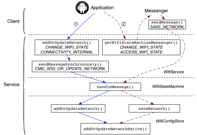
Fig. 4. A motivating case showing inconsistent security enforcement in the Wi-Fi Service of Android 4.4. An app can use either of the two interfaces exposed by the Wi-Fi Service, addOrUpdateNetwork() (call chain connected by solid lines) getWifiStateMachineMessenger() (call chain connected by dashed lines), to update connection configurations to a Wi-Fi access point. However, they are enforcing different permissions. Note that actual call chains have been simplified to better demonstrate the example, with method parameters omitted.
