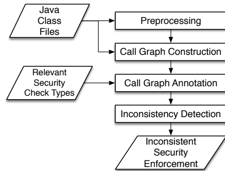
Fig. 7. Kratos analysis flow. There are four major phases: (1) Preprocessing, (2) Call Graph Construction, (3) Call Graph Annotation, and (4) Inconsistency Detection.
