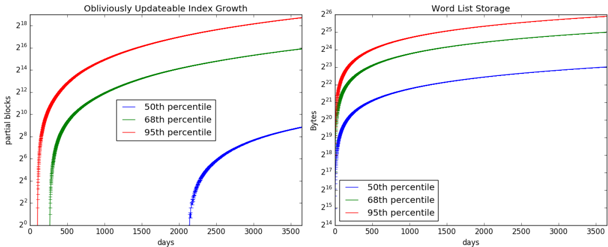
Fig. 7: Simulated long term storage for IO-DSSE. Left: the size of the obliviously updatable index needed (i.e. server side storage) as time goes on for users of different activity levels. Right: the size of the client’s storage under the same conditions.
