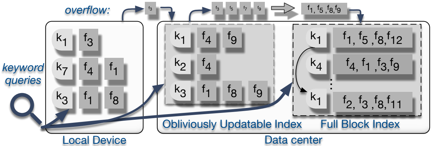
Fig. 1: IO-DSSE logical architecture: an index mapping keywords to document IDs is stored locally, then the largest entries overflow into the obliviously updatable index. When the entry for a keyword in the OUI is full, index entries are inserted into the Full Block Index in chunks. Keyword searches query all three indexes. Note: encryption and the obliviously updatable index construction hide this view from the server.
