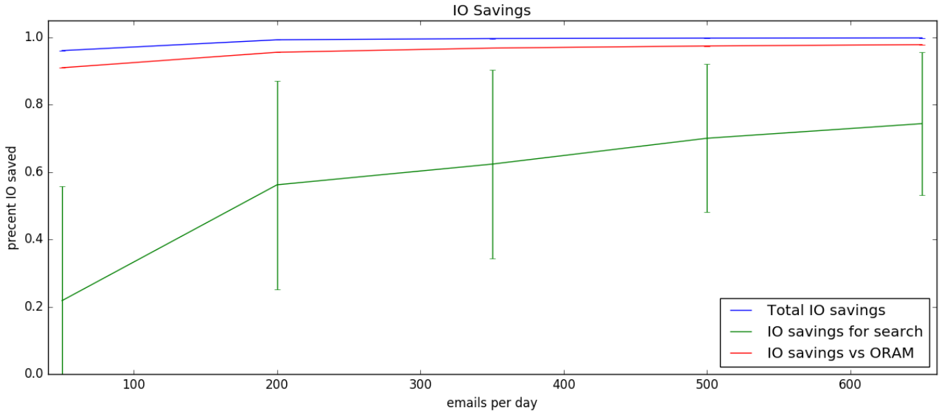
Fig. 6: Experimental and simulated results. IO savings for IO-DSSE vs existing approach and vs an obliviously updatable index constructed with PATH ORAM.
