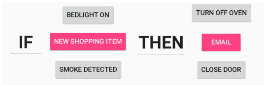
Fig. 5: Inferring user policy via user-driven access control in DTAP. The DTAP-Client enumerates possible triggers and actions. When a user clicks on a specific trigger and action, DTAP-Client automatically treats that as authorization from the user to negotiate rule-specific tokens. There is a one-to-one correspondence between trigger/action names and the scopes.
