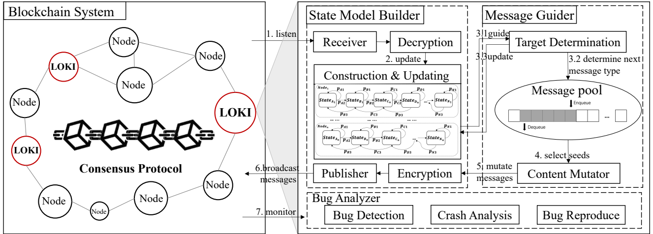
Fig. 4. An overview of LOKI. (1) Module Receiver first listens all the messages, decrypts and analyses them. (2) Next, State Model Builder constructs and updates a state model according to the message sequences. (3) Message Guider determines next message type based on the state model, and updates it. (4) LOKI selects corresponding seeds from the message pool. (5) Content Mutator mutates seeds according to message specifications, and generates new messages. (6) Finally, LOKI encrypts and signs the messages, broadcasts them. (7) The Bug Analyzer monitors the execution information of blockchain system all the time. And LOKI proceeds to the next iteration of the fuzzing process until termination.
