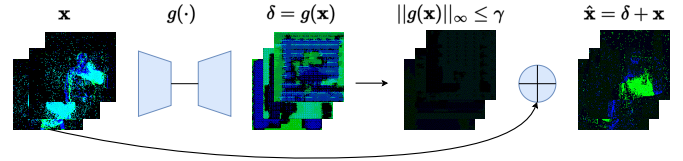
Figure 2: Overview of the dynamic moving attack.
