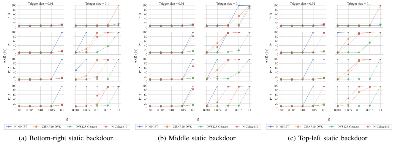
Figure 10: ASR of static triggers.
