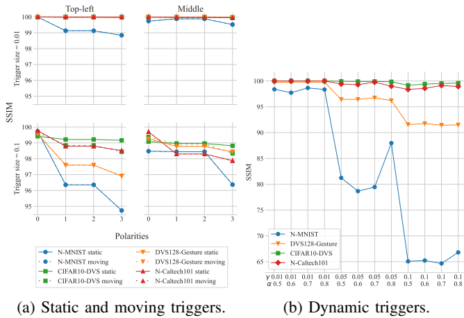
Figure 8: SSIM of different triggers.
