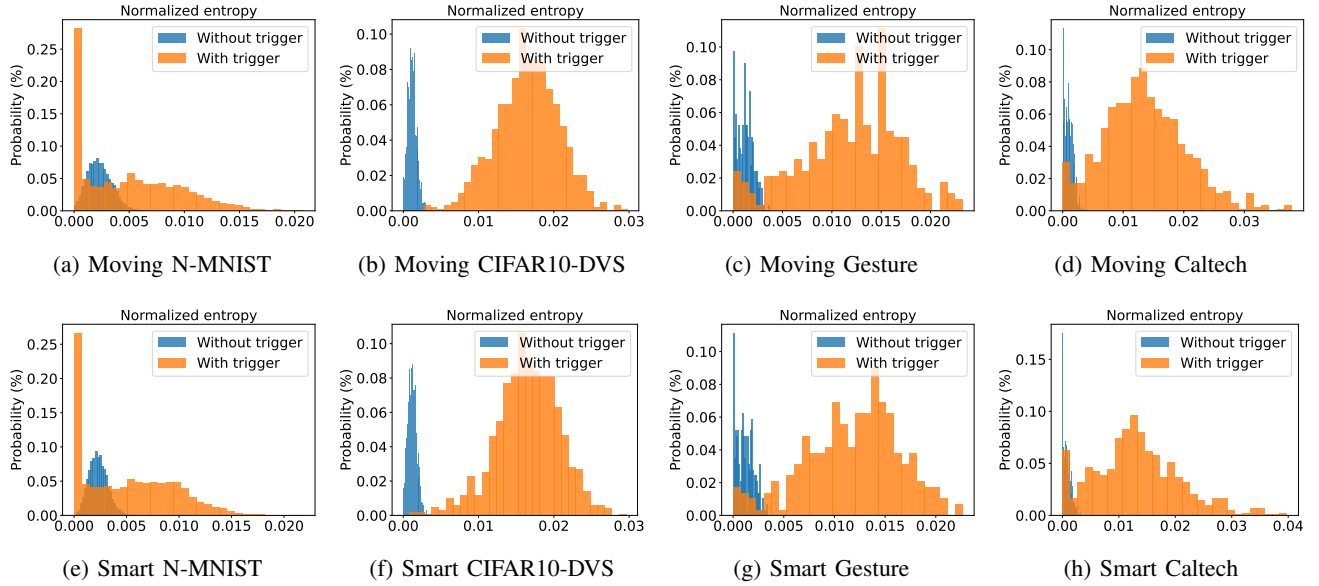
Figure 16: Normalized entropy of different triggers and datasets.
