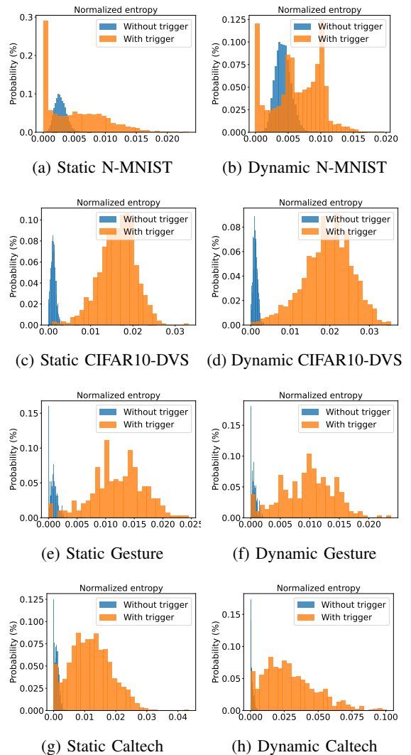
Figure 5: Normalized entropy of different triggers and datasets.
