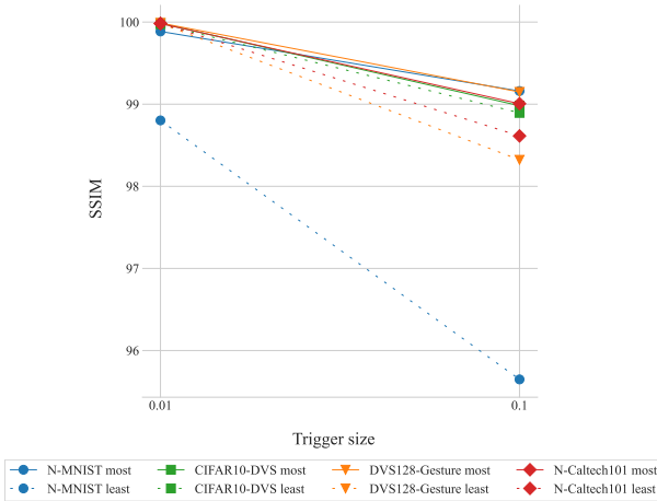
Figure 18: SSIM of smart triggers.
