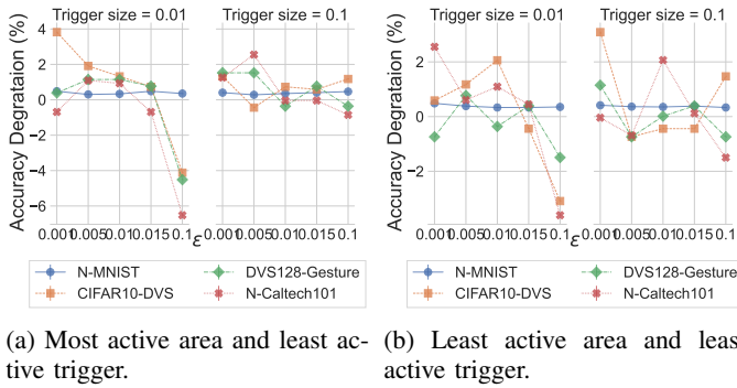
Figure 14: Clean accuracy degradation of the smart trigger in different settings.
