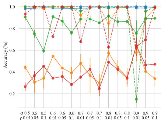
Figure 4: ASR and clean accuracy degradation of dynamic triggers. Dashed lines represent the ASR, and solid lines represent the clean accuracy. Blue corresponds to N-MNIST, orange to CIFAR10-DVS, green to DVS128-Gesture, and red to N-Caltech101.
