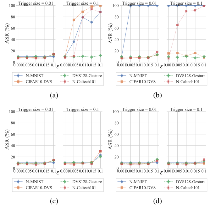
Figure 3: 3a and 3b show the smart triggers in the most active area, using the least and most common polarity. In 3c and 3d, we show the smart triggers in the least active area, using the least and most common polarity.
