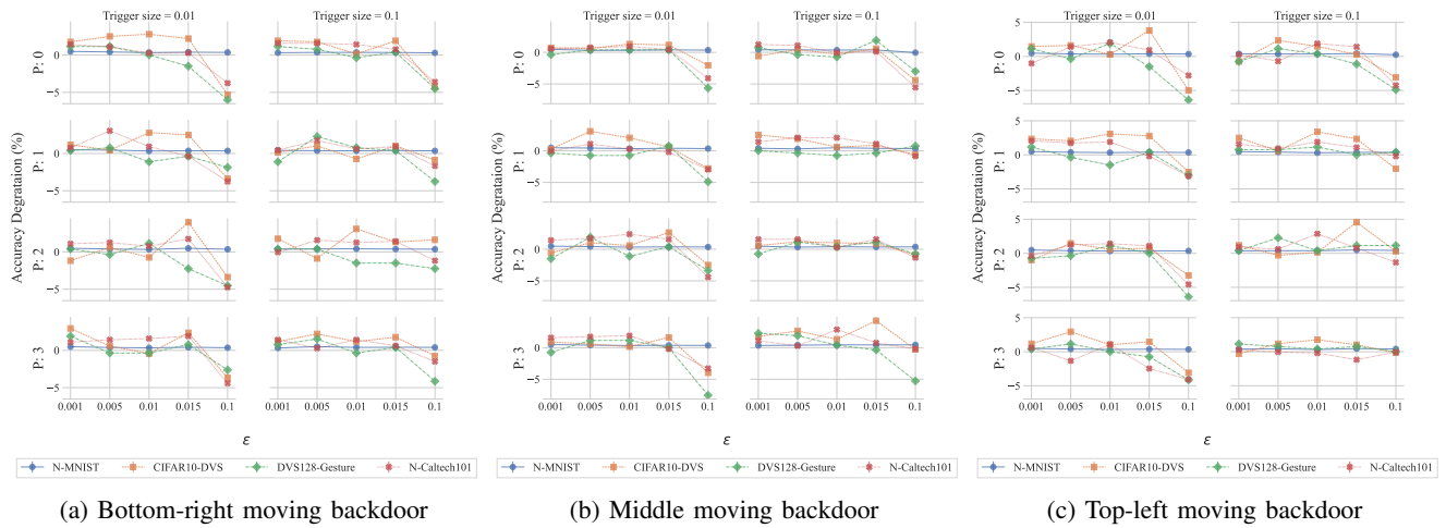
Figure 13: Clean accuracy degradation of moving triggers.
