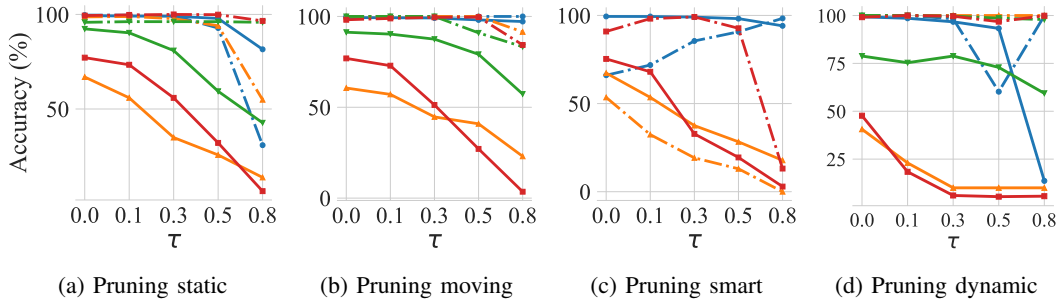
Figure 17: Effect of pruning on the ASR (dashed lines) and clean accuracy (full line) for different types of attacks, i.e., static, moving, smart, and dynamic. Blue corresponds to N-MNIST, orange to CIFAR10-DVS, green to the DVS128-Gesture, and red to N-Caltech101.
