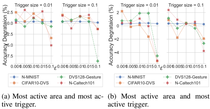
Figure 15: Clean accuracy degradation of the smart trigger in different settings.
