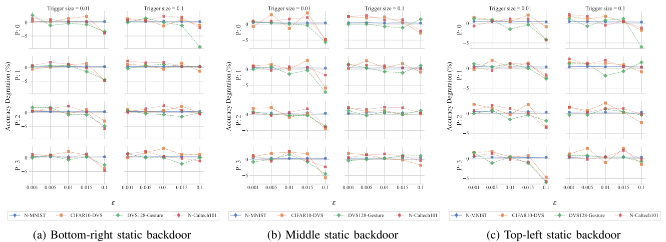
Figure 12: Clean accuracy degradation of static triggers.
