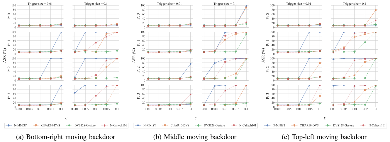
Figure 11: ASR of moving triggers.
