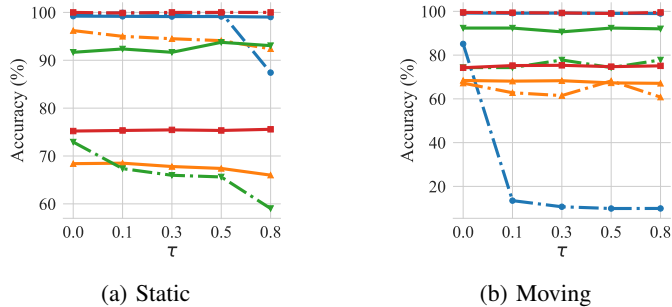
Figure 7: Results of different adaptive attacks after fine-tuning. ASR (dashed lines) and clean accuracy (full line) for different types of attacks, i.e., static and moving. Blue corresponds to N-MNIST, orange to CIFAR10-DVS, green to DVS128-Gesture, and red to N-Caltech101.
