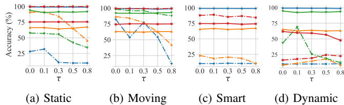
Figure 6: Effect of fine-pruning on the ASR (dashed lines) and clean accuracy (full line) for different types of attacks, i.e., static, moving, smart, and dynamic. Blue corresponds to N-MNIST, orange to CIFAR10-DVS, green to DVS128-Gesture, and red to N-Caltech101.
