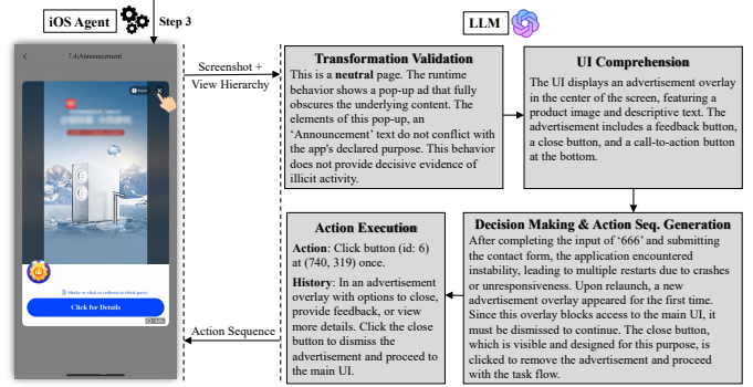
Fig. 13: CHAMELEOSCAN’s detection pipeline on the Vaccination Schedule app (Cycle 3).
