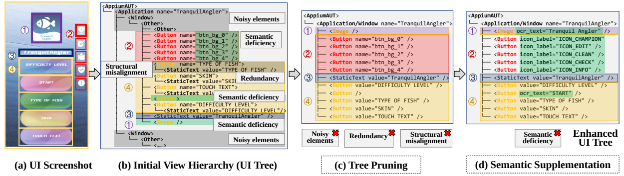
Fig. 6: View hierarchy (UI tree) enhancement procedure demonstrated using the “Tranquil Angler” app.
