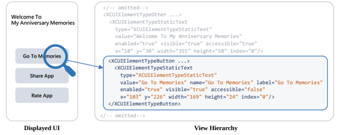
Fig. 2: UI screenshot and view hierarchy (partial) of an app.
