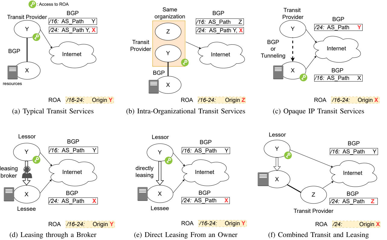
Fig. 2: Misconfigured ROA scenarios due to mismatches between the ROA origin and BGP origin. They can occur when an AS uses a transit provider (a, b, c), leases IP prefixes either through a broker or directly from a lessor (d, e), or combines both leasing and transit services (f). Notably, only scenario (a) can be readily identified through BGP relationships because both the customer and provider appear in the AS_PATH, and prior studies have focused almost exclusively on this case [9], [59], [26]. Please refer Appendix §IV-D for real-world examples of each hidden type of ROA misconfigurations.
