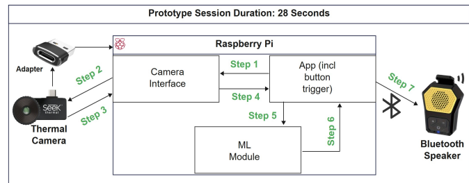
Fig. 1. Security Architecture Diagram
