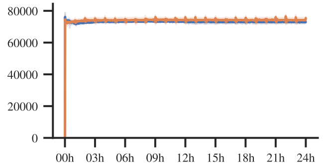
Figure 5: Executions per second over 24 hours for zlib (8 cores) for baseline AFL++ (●) and POGFUZZ (●)
