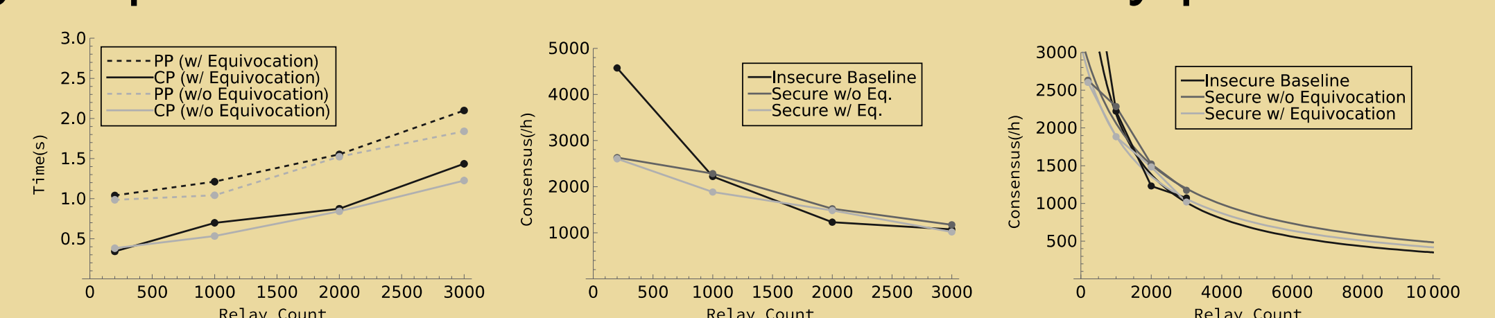
Figure 8: Average network and CPU time for different phases of our protocol. PP - Bootstrap Phase, CP - Agreement Phase. Figure 9: Network throughput in three test scenarios, measured in consensus per hour. Figure 10: Prediction of throughput up to 10,000 relays. The protocol can generate up to 500 consensus documents per hour.
